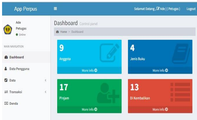
Gambar 14 Halaman Admin
