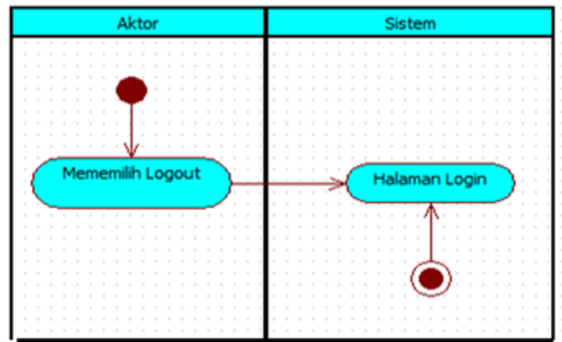
Gambar 6 Activity Diagram Logout
